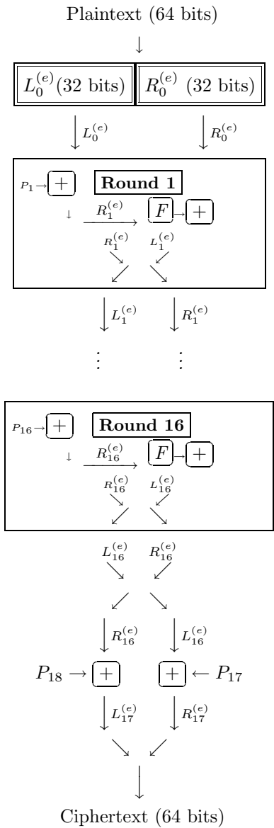
Diagram 3.4 Blowfish Encryption
