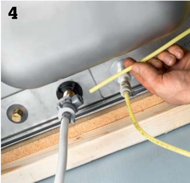
4 Cut lengths of tubing to run between the water supply, filter unit, and spout, making sure the cuts are square and the tubing ends are free of scratches, kinks, and rough spots. Connect the tubing at the push-in (or other) fittings. Test and flush the system as directed.
