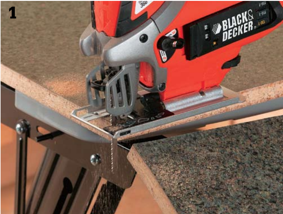
OPTION: Use a jigsaw fitted with a downstroke blade to cut post-form. If you are unable to locate a downstroke blade, you can try applying tape over the cutting lines, but you are still likely to get tear-out from a normal upstroke jigsaw blade.
