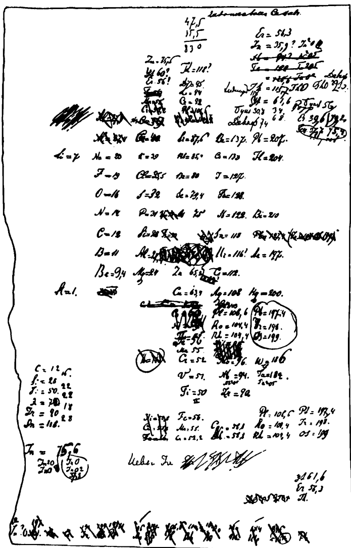
Figure 6.1 Mendeleev's first draft of the periodic table of the elements.
