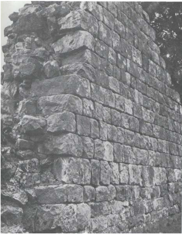
A fragment of the structure of Hadrian's Wall at Hare Hill; the core is original, and the facing stones are restored.
