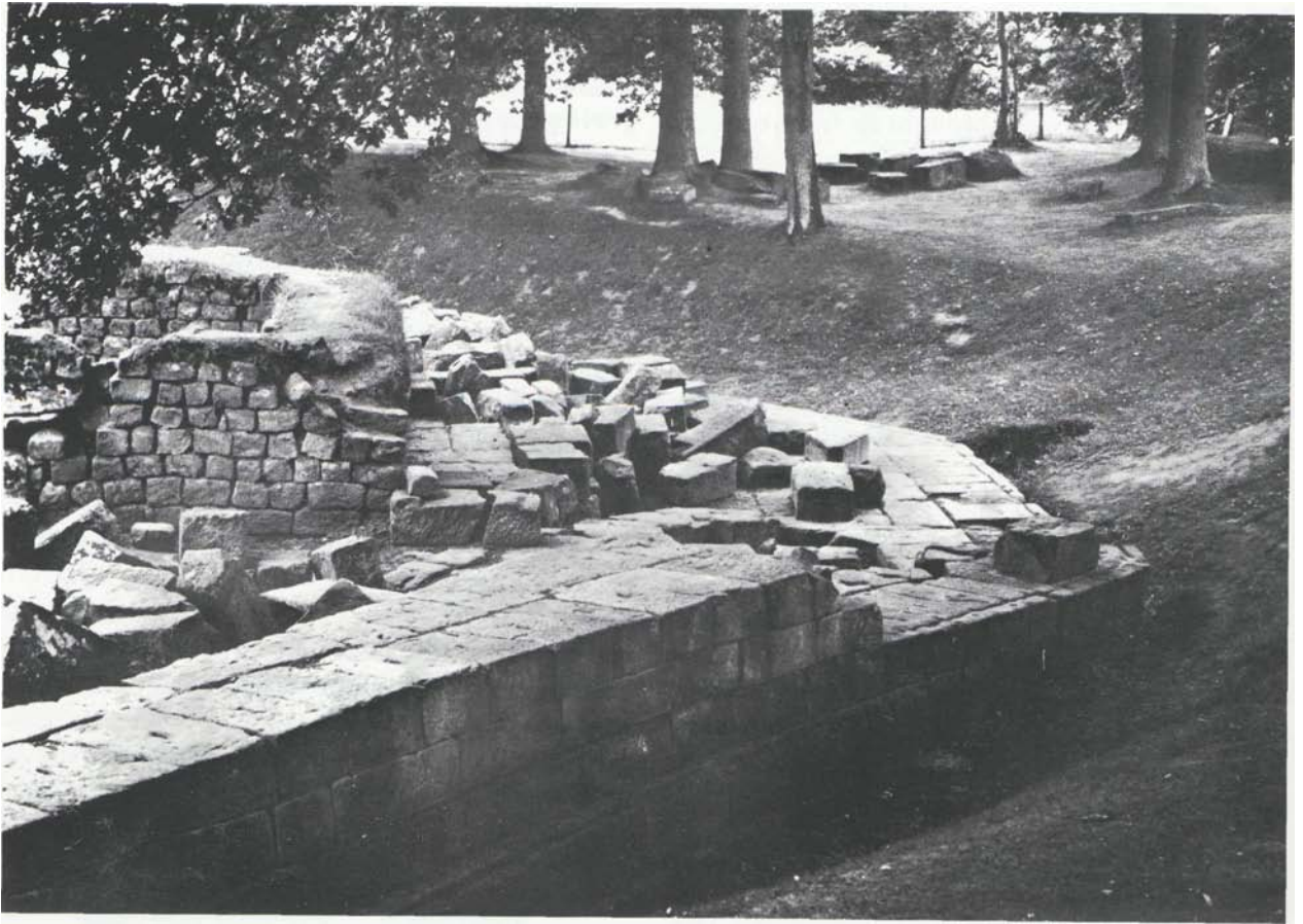
The bridge abutment at Chesters, where the Wall crosses the North Tyne; in some of the stone blocks 'Lewis holes' are still clearly visible.
