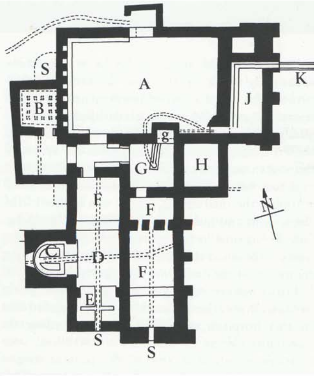
The bath-house at Chesters Fort: (A) Changing and recreation room (B) Hot room—hypocaust (C) Hot bath (D) Hot room (E) Water boiler (F) Warm rooms (G) Cold room (g) Cold plunge (H) Cold bath (J) Latrine (K) Outflow to river (S) Stoke-holes.
